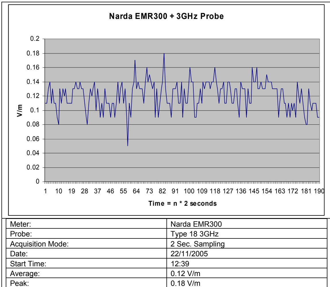
Fig 16: Measurements recorded in the hot press
