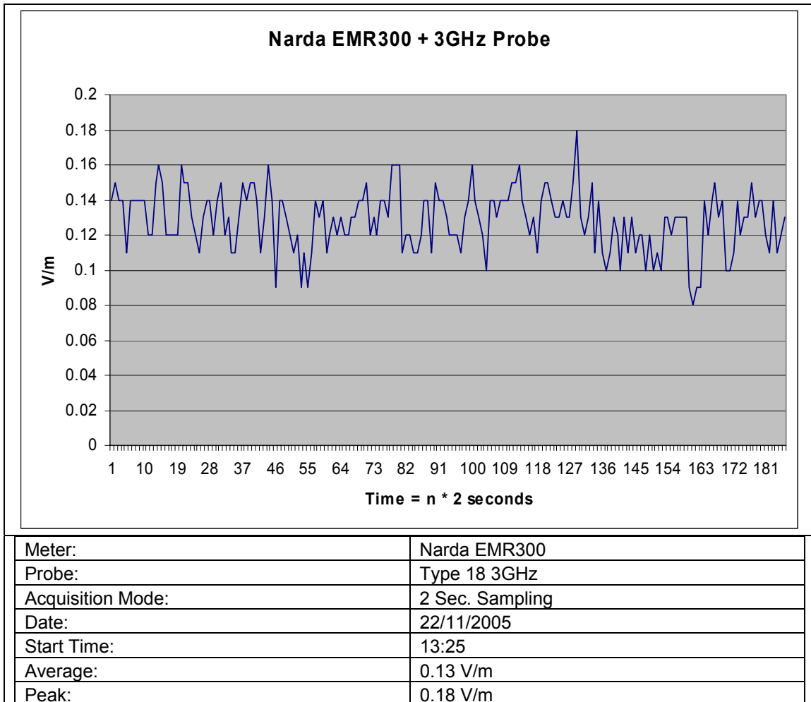
Fig 14: Measurements recorded beside Television
