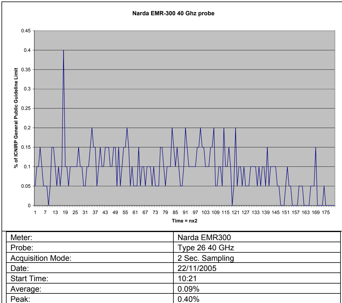
Fig 2. Measurement as a percentage of the ICNIRP general public guideline limit recorded over a 6 minute period using the 40GHz probe
