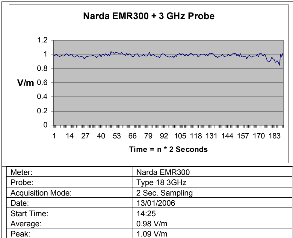
Fig 1. Field strengths recorded over a 6 minute period using the 3GHz probe
