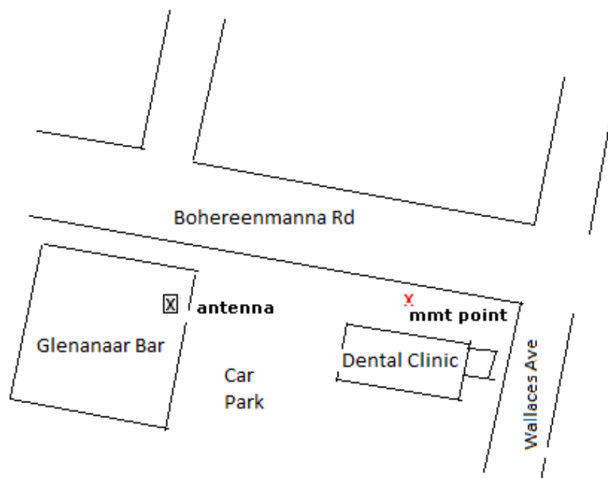
Map of Transmitter Site and Measurement Location
