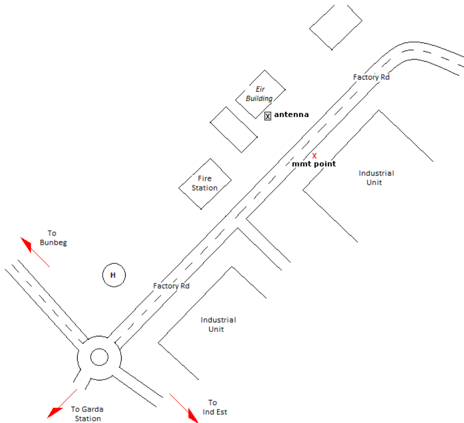
Map of Transmitter Site and Measurement Location
