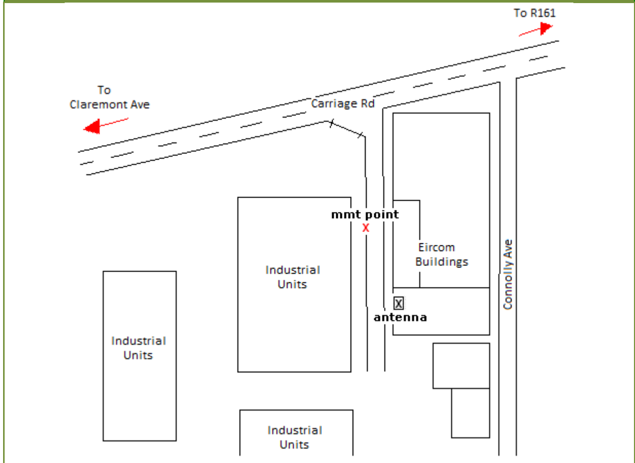
Map of Designated Transmitter Site and Measurement Location
