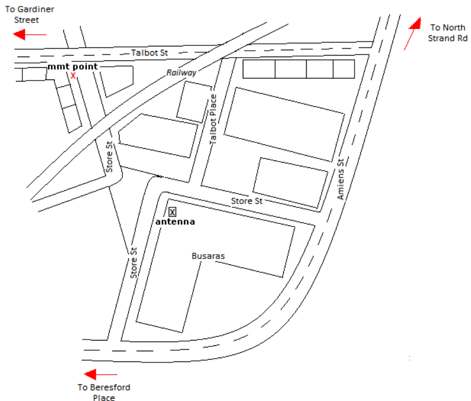
Map of Designated Transmitter Site and Measurement Location
