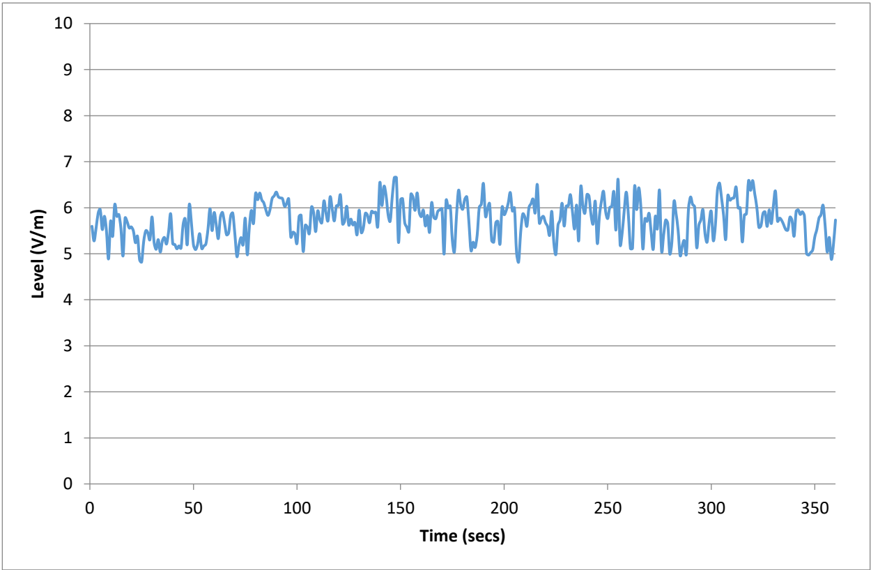
Electric field strengths recorded over 6 min period using 40 GHz probe at point of maximum NIR
