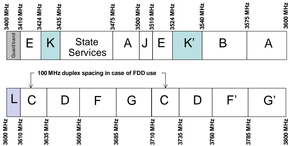
Figure 1: 3.4 GHz – 3.8 GHz frequency band
